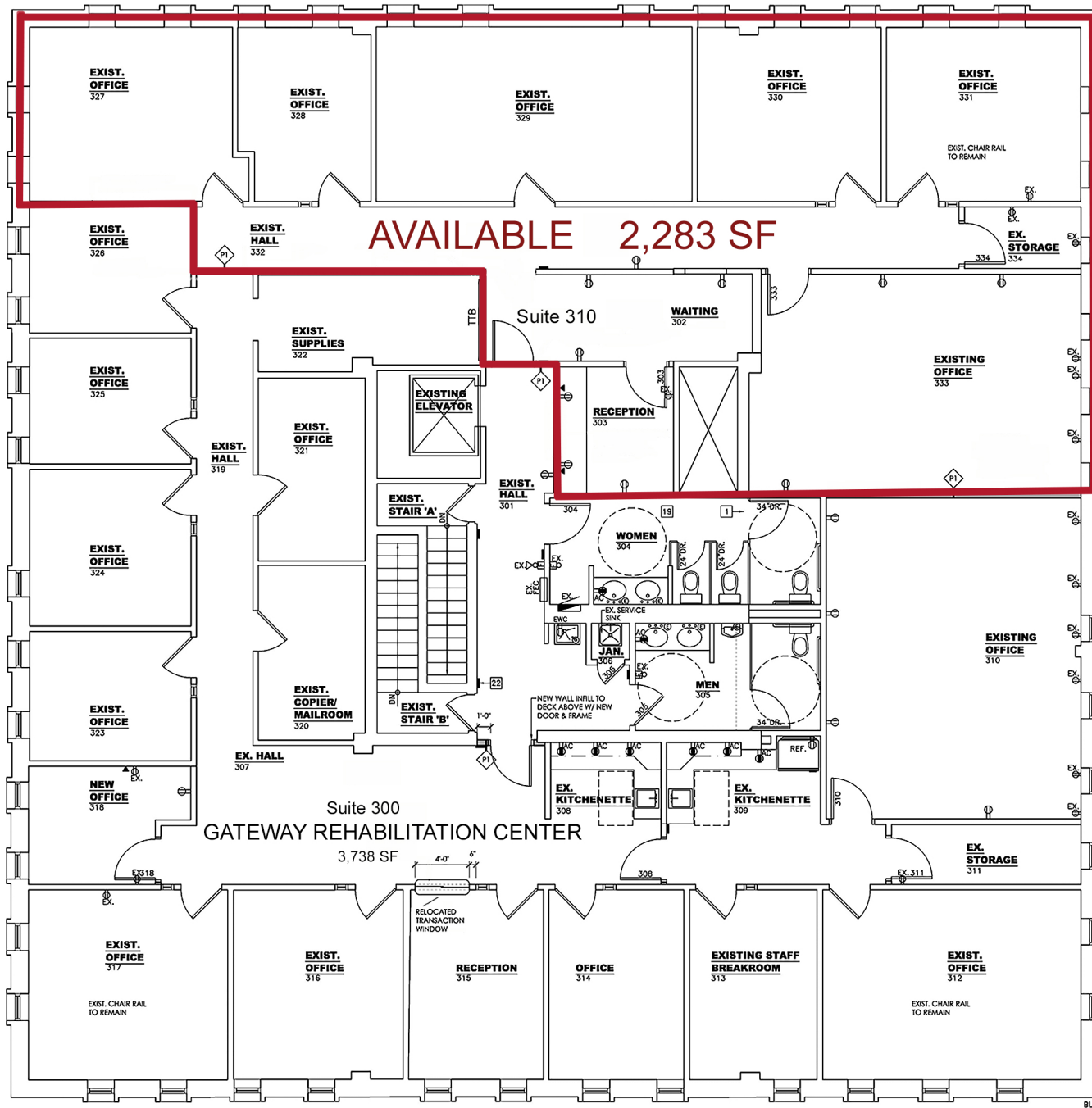
1 THIRD FLOOR PLAN SCALE: 1/4"=1'-0"
