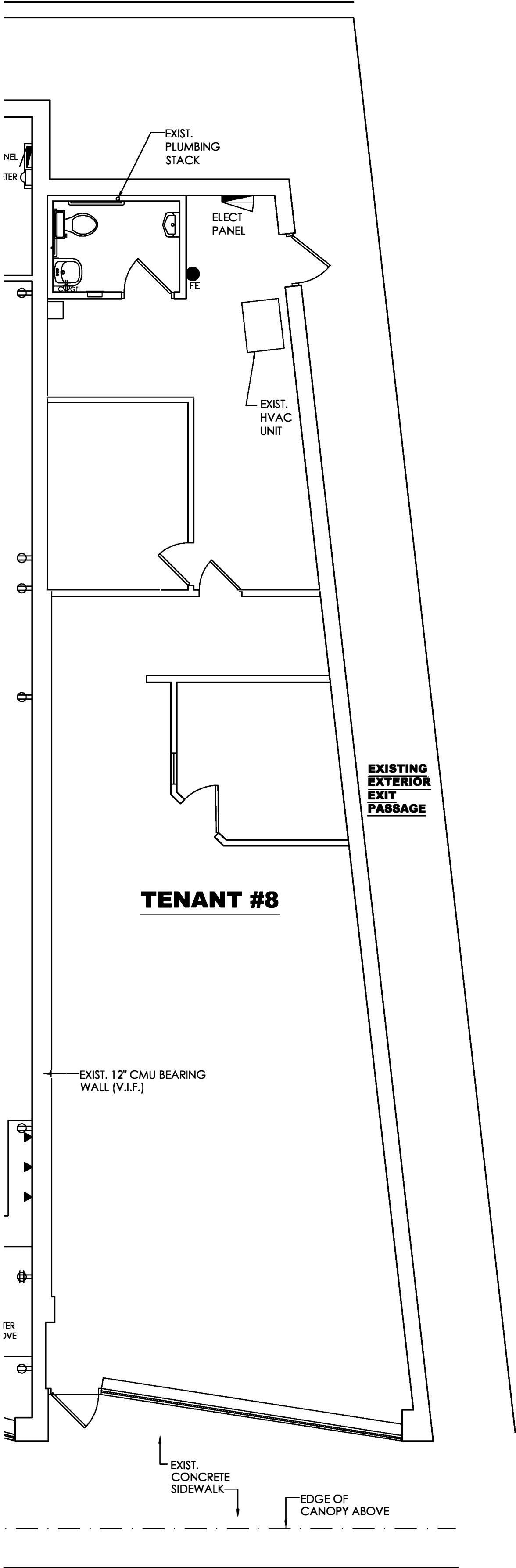
EXISTING FLOOR PLAN SCALE: 3/16"=1'-0"
