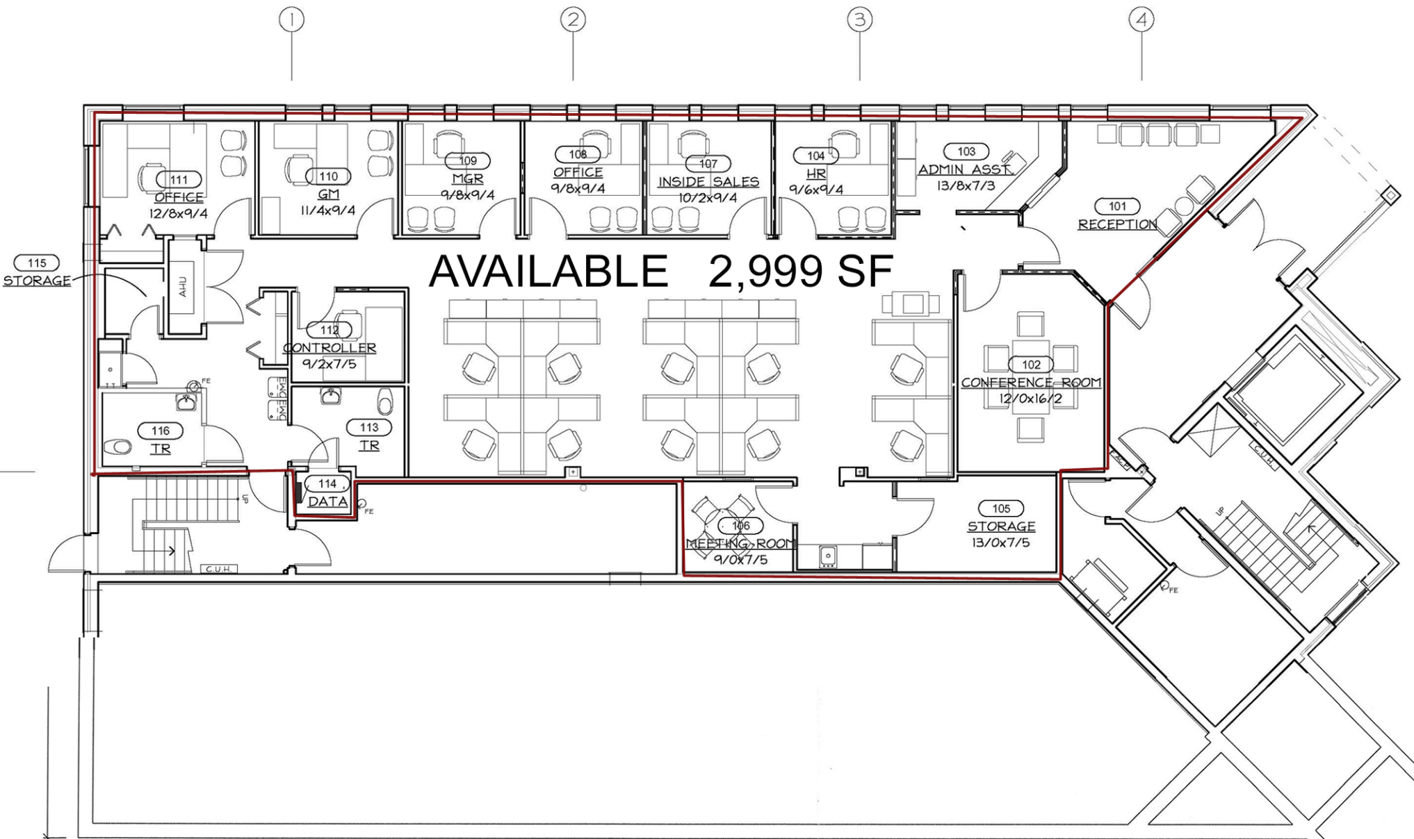
1 Ground Floor Plan G Scale: 1/8"=1'-0"
